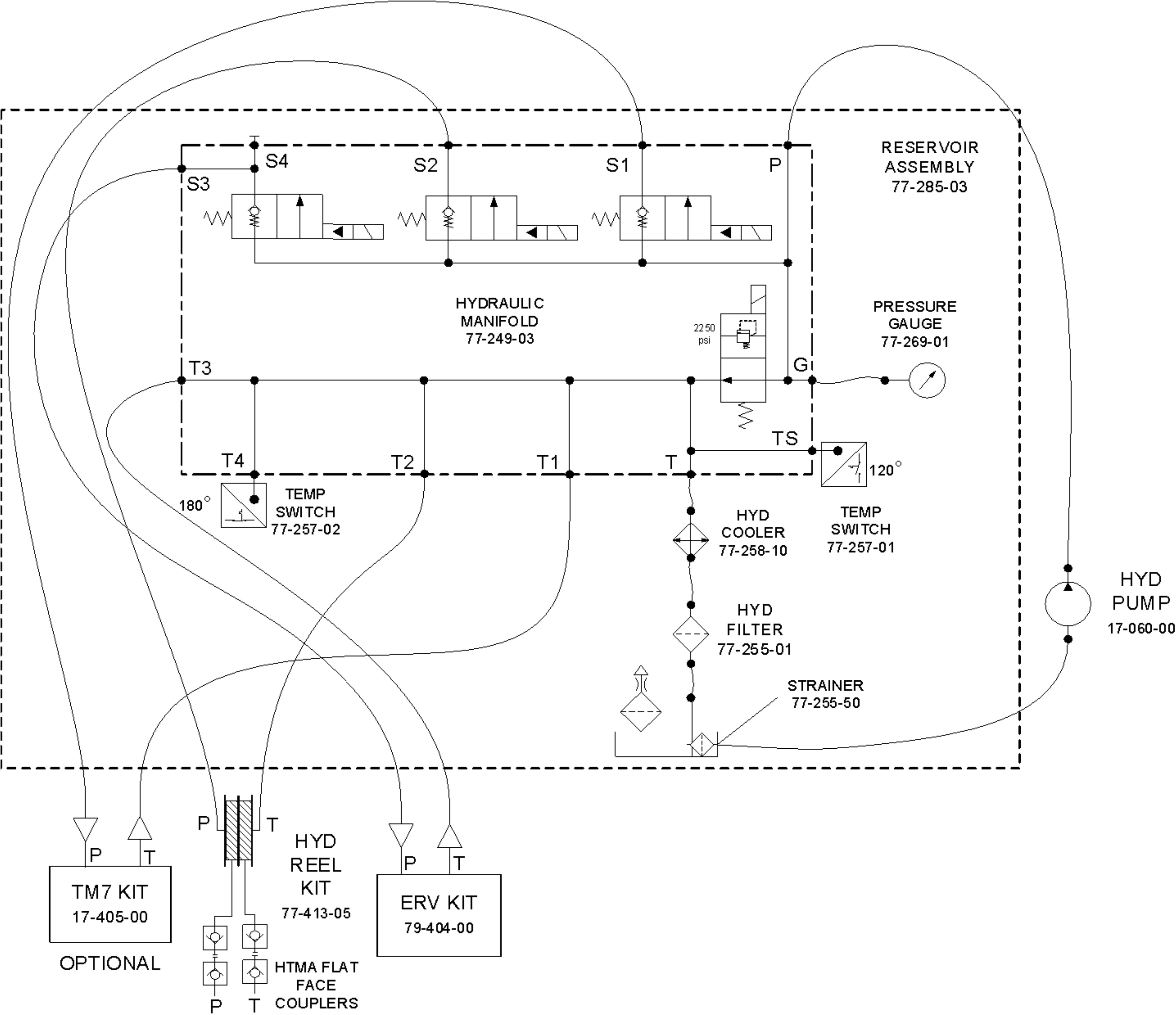
HYDRAULIC SCHEMATIC
